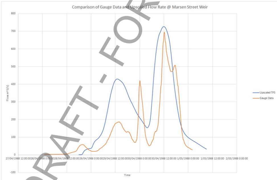
Figure 7-3 Comparison of gauge data and upscaled 1% AEP 12hr TP5 TUFLOW result at MarsenMarsden Street weir (15%+)
