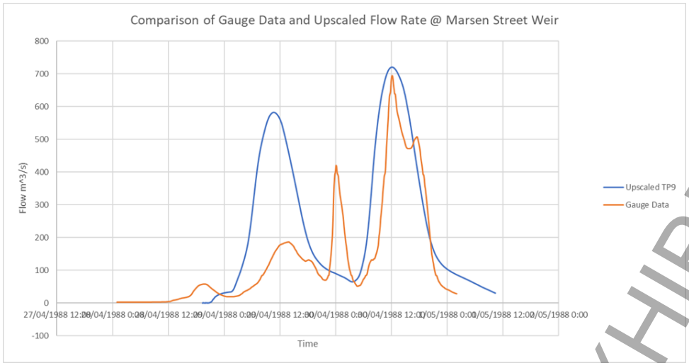
Figure 7-1 Comparison of gauge data and upscaled 1% AEP 12hr TP9 TUFLOW result at MarsenMarsden Street weir (8%+)
