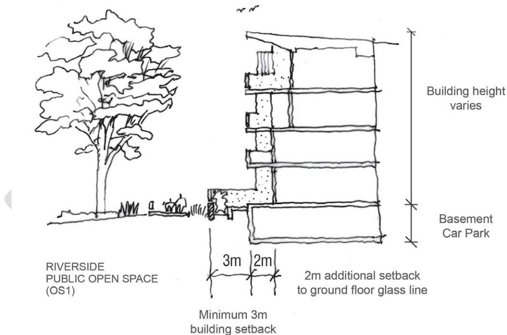
Figure 8.2.2.12.5.1 - Typical Riverside Section
