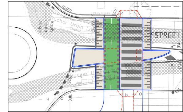
Gray Street refuge island proposed upgrade to priority pedestrian and cyclist crossing.
