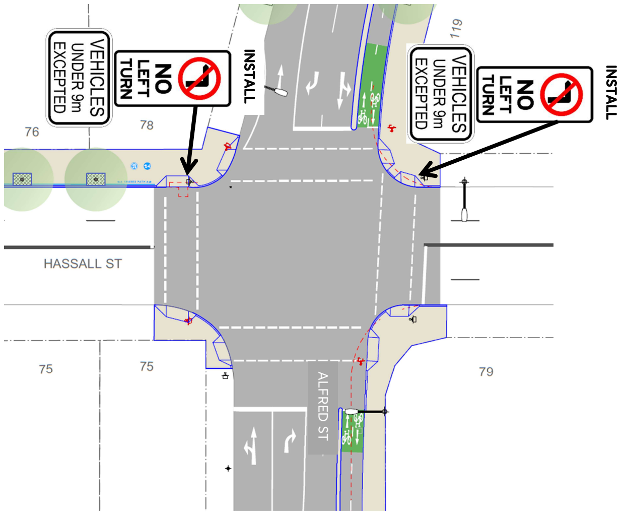
Figure 1: Proposed turn restriction at Alfred Street and Hassall Street
