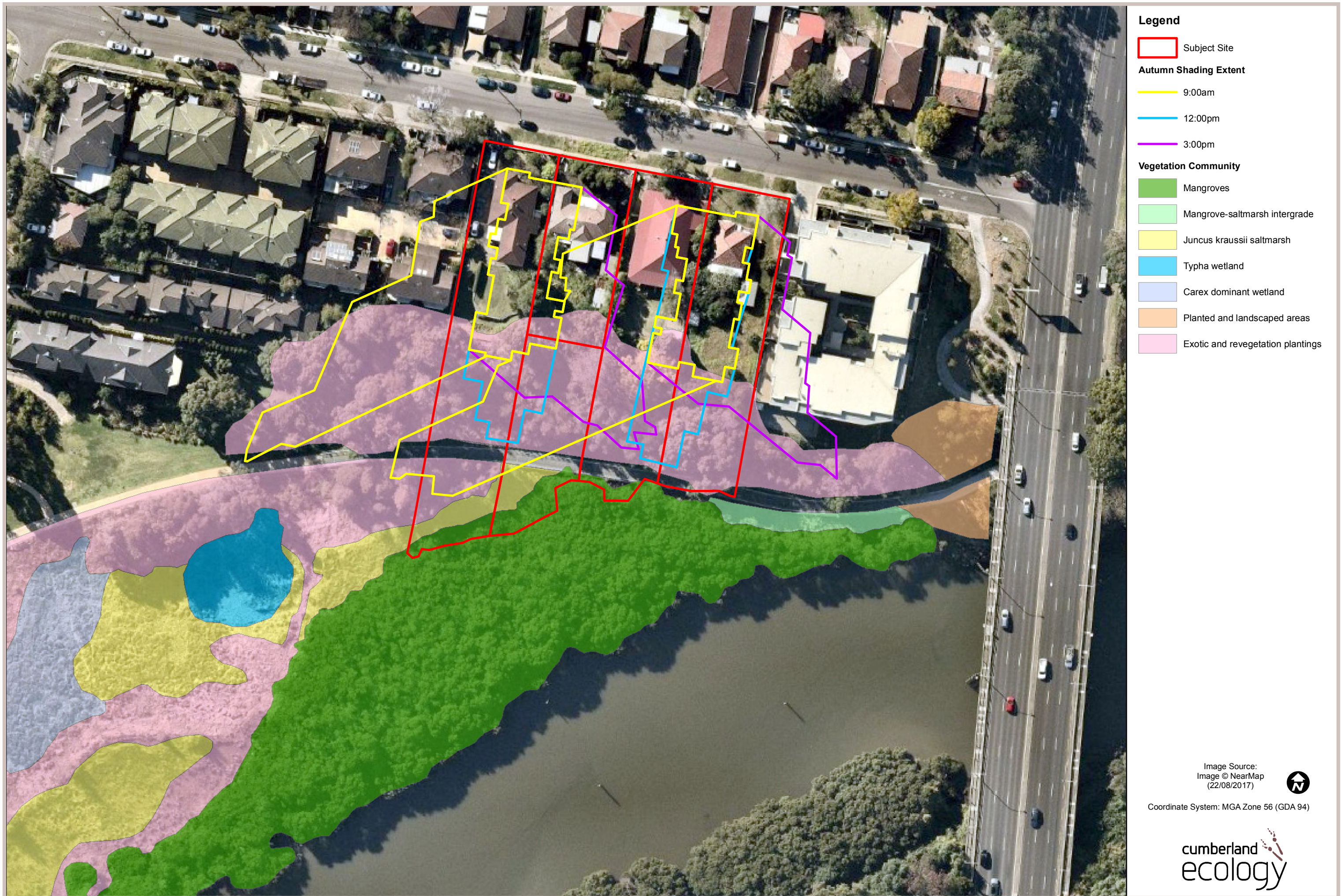
Figure 3.13. Shading Extent of Vegetation Communities during Autumn
